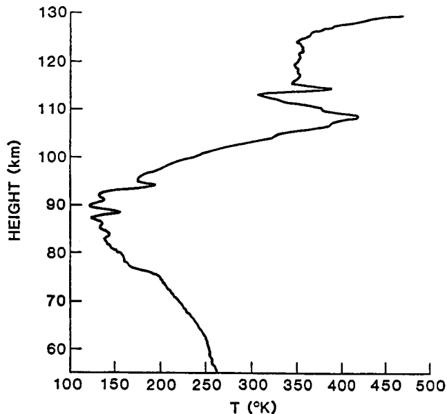
Figure 4. Temperature profile obtained by accelerometer sphere at 2055 AST, June 15, 1983. Note the cold summer mesopause with a temperature of 130°K near 86 km.
